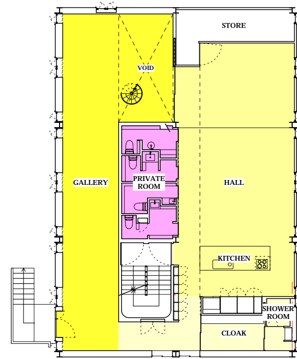
2F PLAN (1/200)
